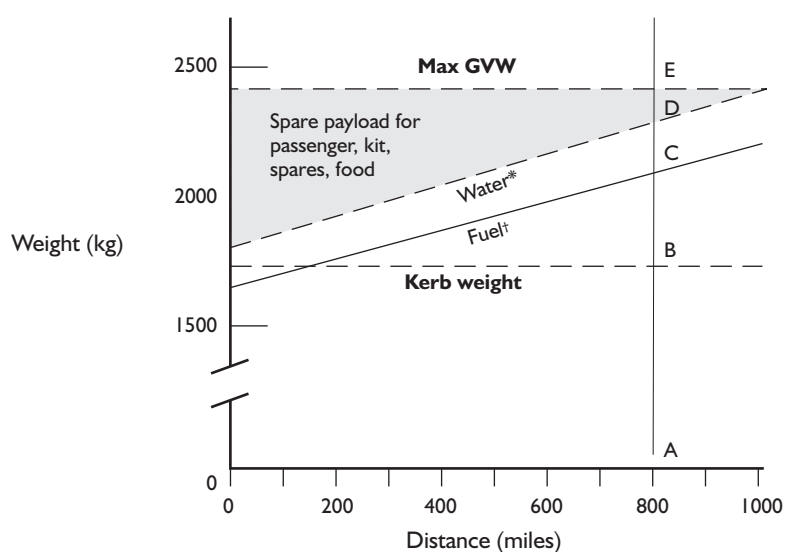
Figure 28.2 Payload versus range. This graph, for a V8 Defender 90, shows vividly how operating range (distance between replenishment points) erodes spare payload. In a fairly extreme case, on an 800-mile leg, A–B is kerb weight, B–C is fuel load, C–D is water required, leaving only 150 kg (D–E) for a 75-kg passenger and remaining kit. In real life you would go diesel, shorten legs and/or get a bigger vehicle such as the Land Rover Defender 110 or a robust 4 × 4 pickup such as a Toyota Hilux. Fuel calculations assume reserve, i.e. distance + 100 miles + 25 per cent. Bigger vehicle equals more payload but less power:weight ratio (see Figure 28.6).
