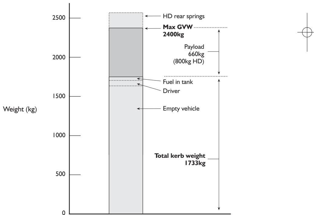
Figure 28.1 How a vehicle's GVW (gross vehicle weight) is made up. Never exceed it by adding too much payload. Figures shown are for Defender 90
